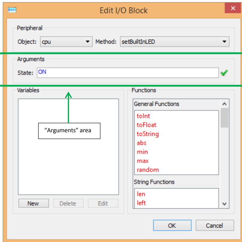
Figure 2-20: Edit I/O Block dialog
