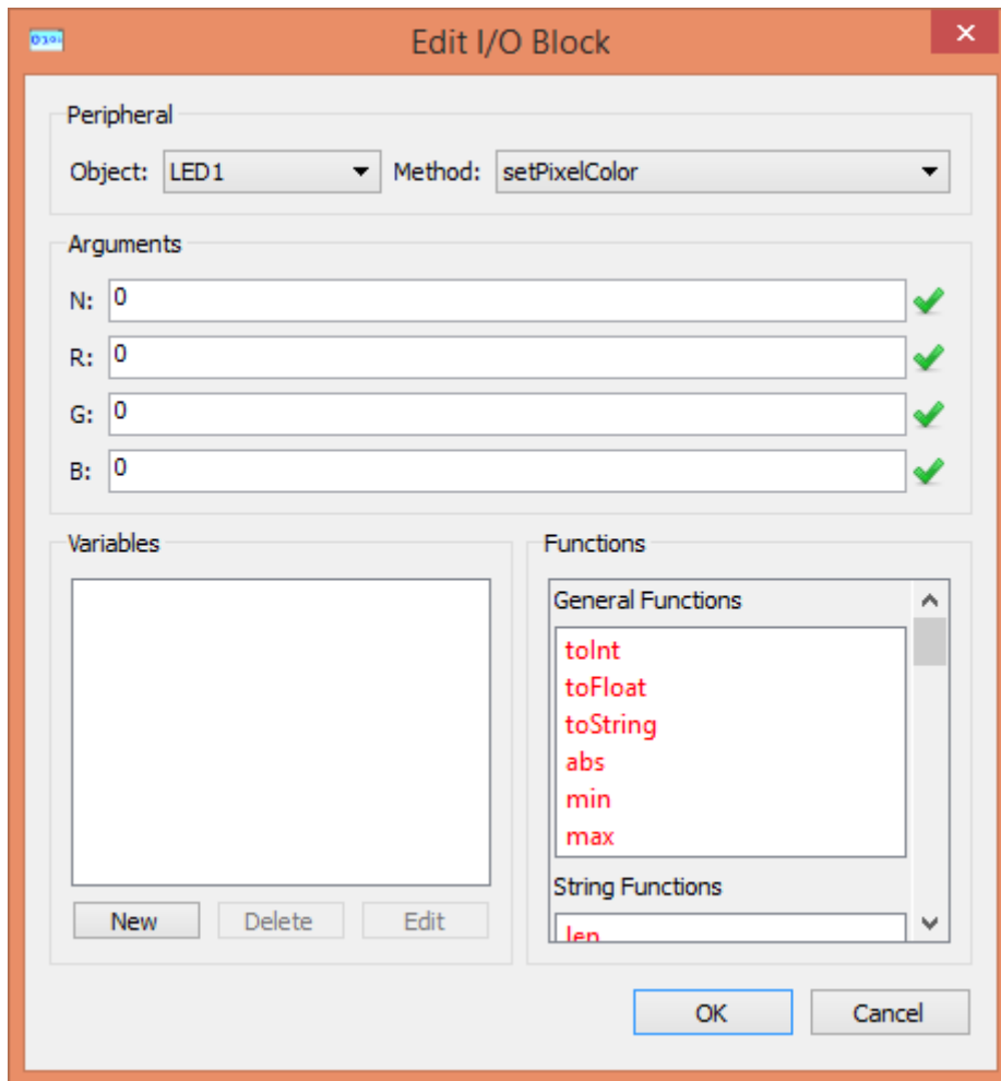
Figure 8-4: Edit I/O block dialogue for the setPixelColor method
