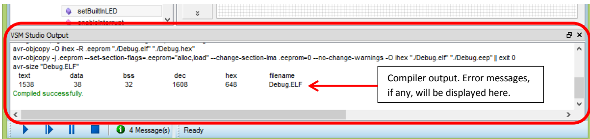
Figure 2-25: Compiler output
