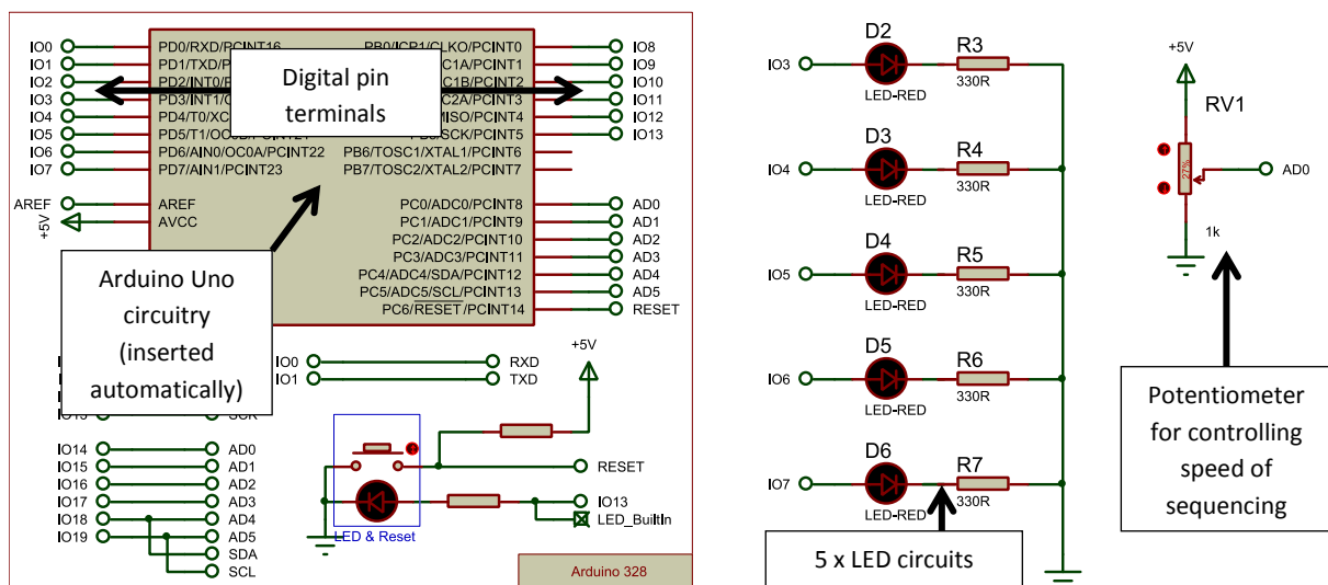
Figure 7-2: Sequencing LEDs circuitry
