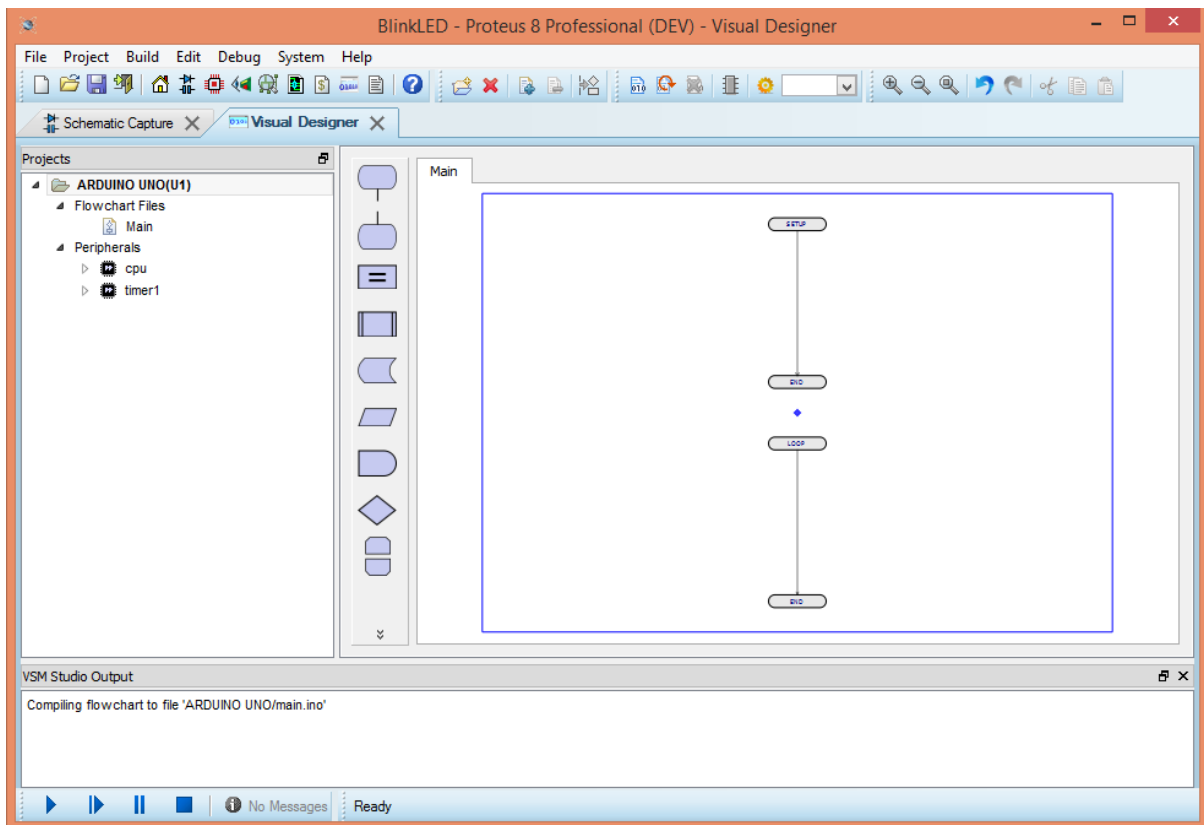
Figure 2-5: New flowchart project
