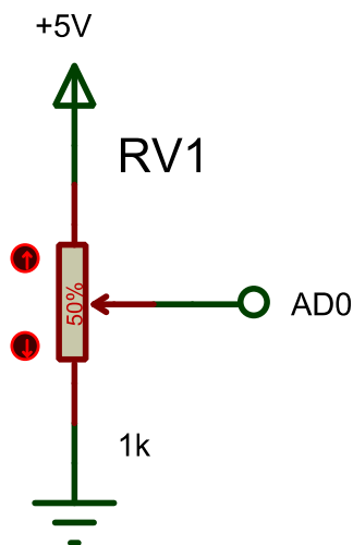
Figure 7-6: Potentiometer circuit
