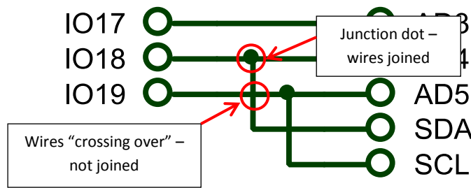
Figure 6-18: Junction dots
