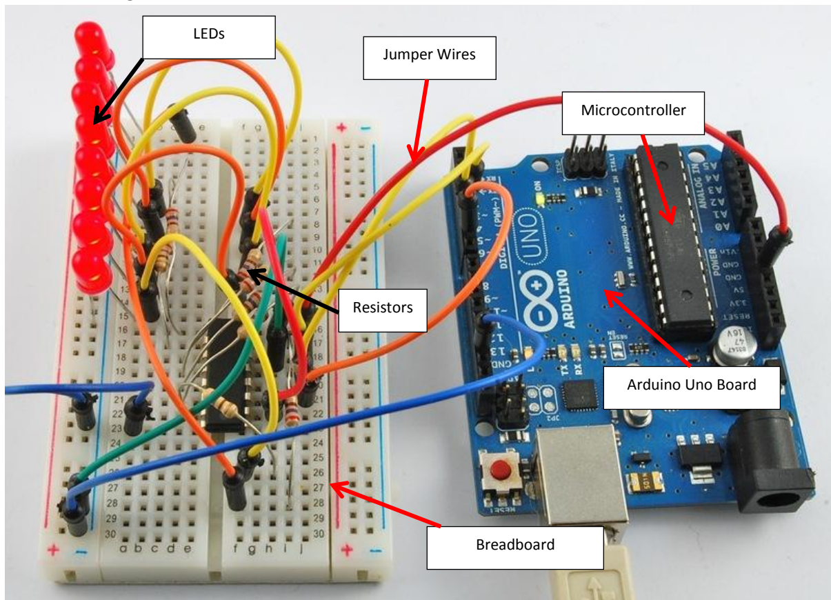
Figure 7-1: Breadboarding 16
