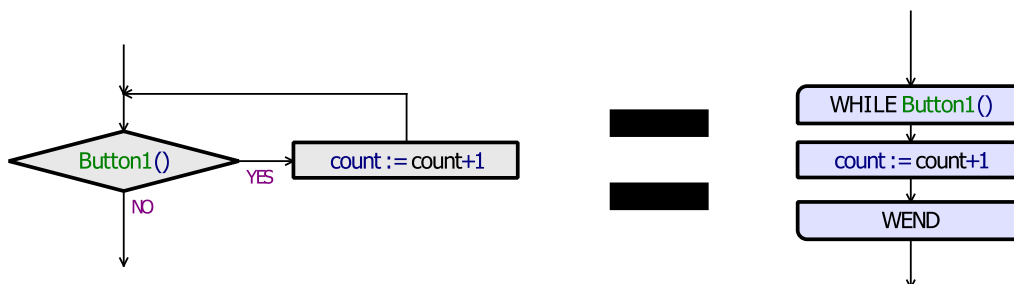
Figure 8-11: While-Wend loop
