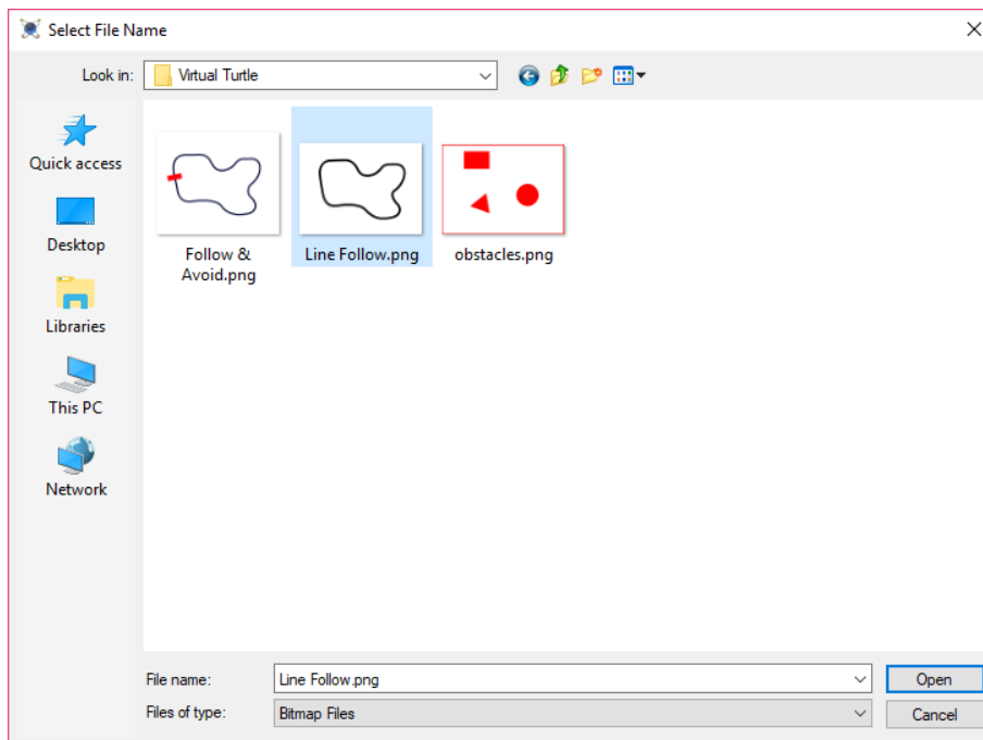
Figure 11-20: "Browse" dialogue
