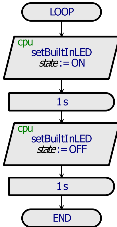
Figure 2-11: Blink LED flowchart
