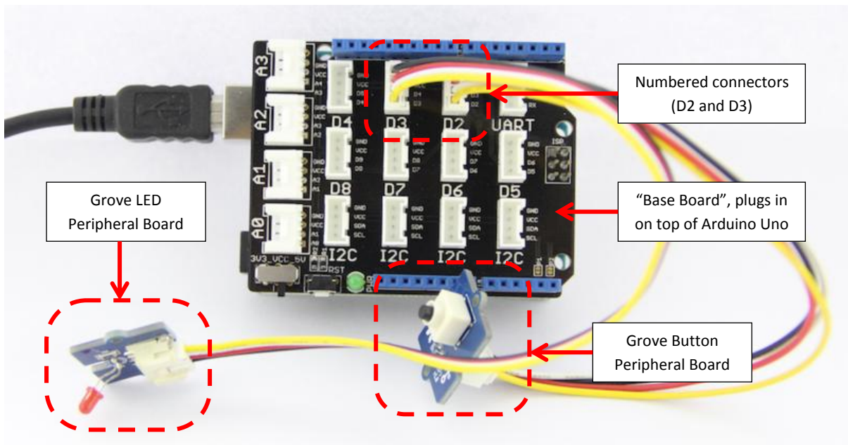
Figure 3-16: Grove System 8
